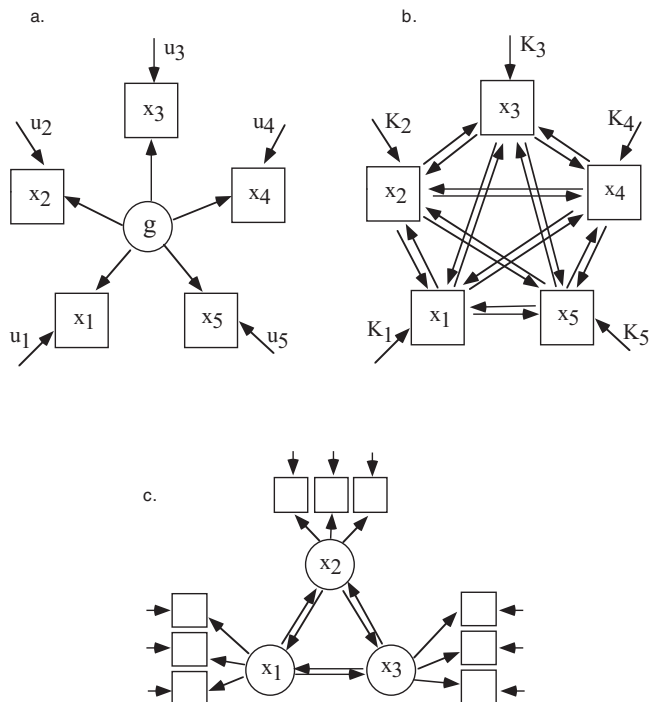
Figure 1. Three models of the positive manifold: (a) the standard g model, (b) the mutualism model, and (c) the extended mutualism model. Squares and circles denote manifest and latent variables, respectively. Symbols x denote processes, u unique variances, and K resources (see text).
